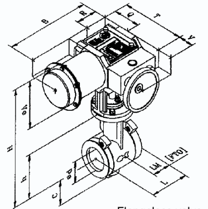
Flangeless valve "Sandwich" Actuator P/R-99-1
