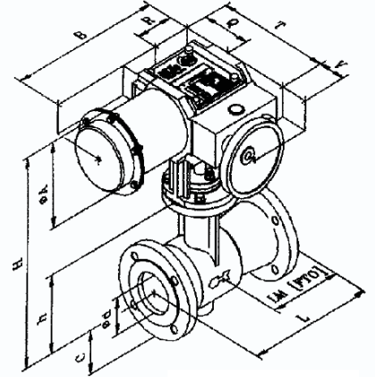
Flanged valve Actuator P/R-99-1
